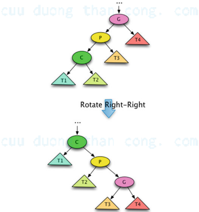
Fig. 10.10 Splay Tree Double-Right Rotate
