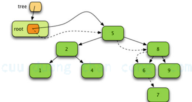
Fig.6.11 The Tree After Inserting 7
