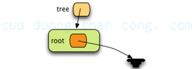
Fig. 6.3 An empty BinarySearchTree object
