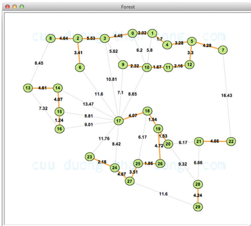
Fig. 7.7 Kruskal's: Snapshot 2
