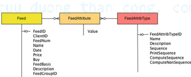
Fig. 11.3 Logical Data Structure
