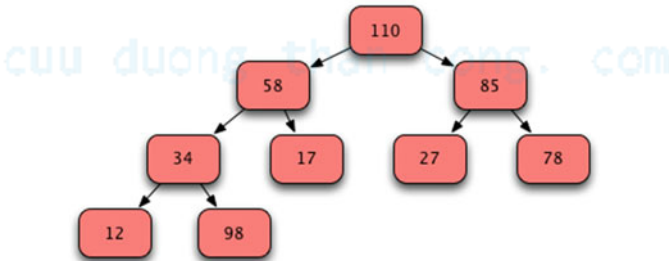
Fig. 9.8 Conceptual View While Adding 98 to the Heap
