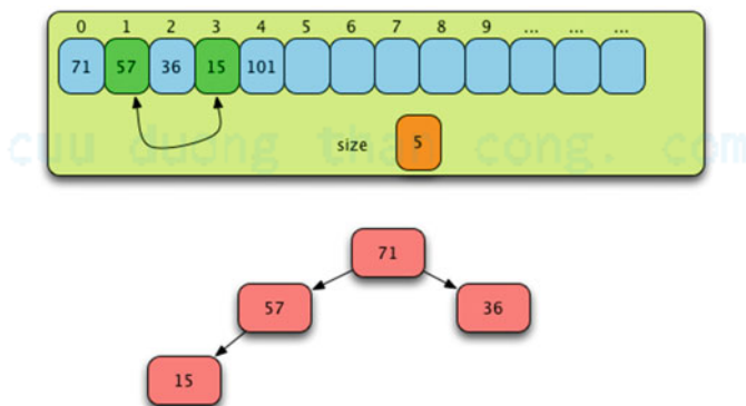
Fig. 9.4 Building a Heap Part One
