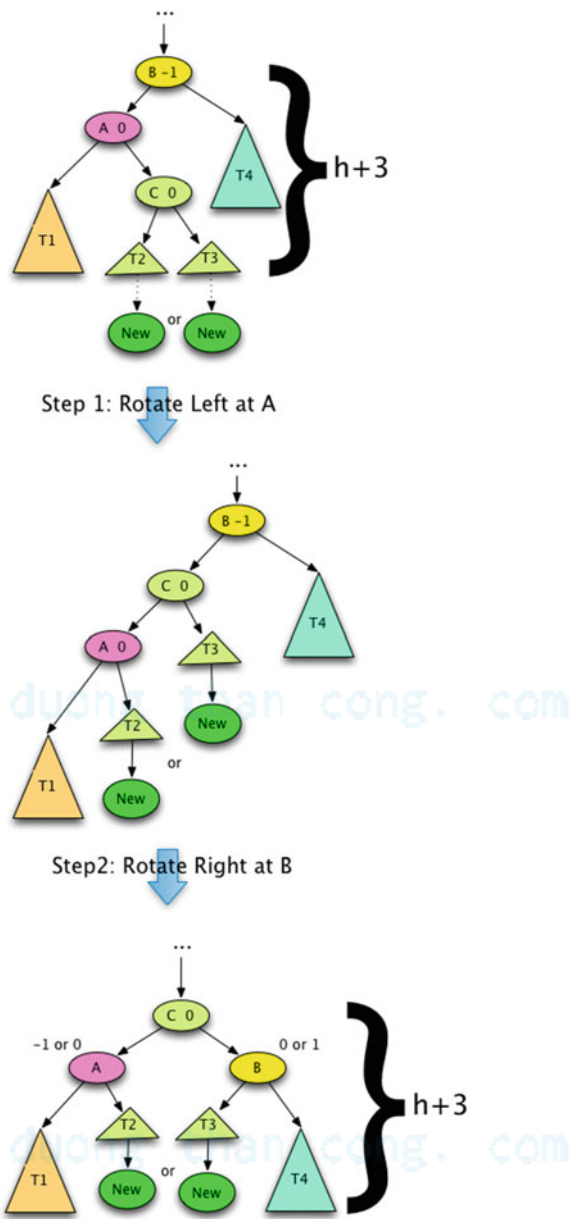
Fig. 10.9 AVL Tree Case 3B Steps 1 and 2
