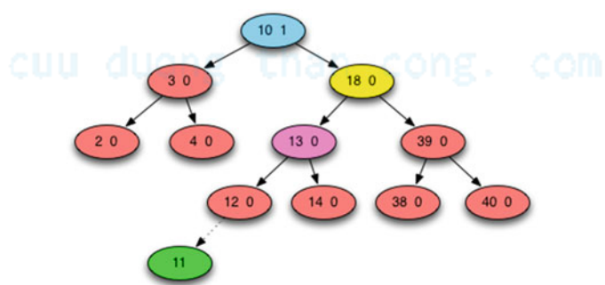
Fig. 10.4 AVL Tree Case 3B—Double Rotation
