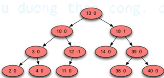
Fig. 10.6 AVL Tree Case 3B Step 2 Rotate Away
