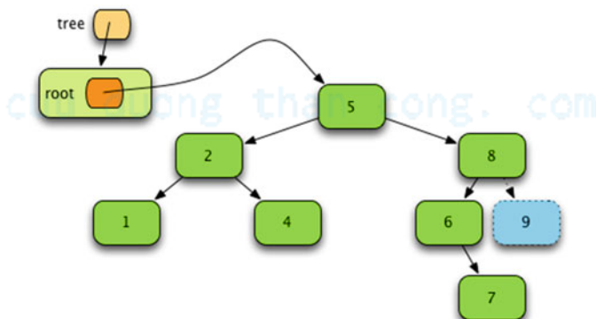
Fig. 6.13 The Tree After Deleting 9
